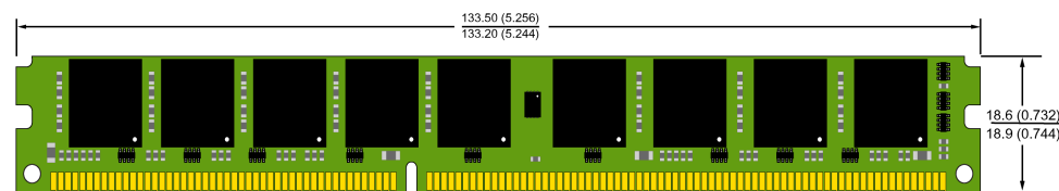
UDIMM VLP MO-269 240 PIN
