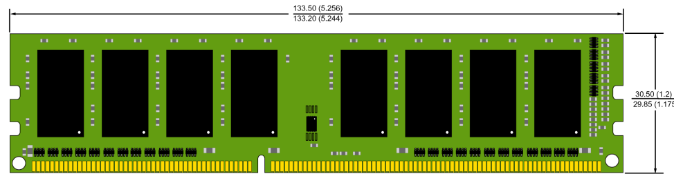
UDIMM MO-269 240 PIN
