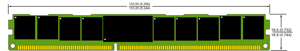
LR-DIMM VLP MO-269 240 PIN
