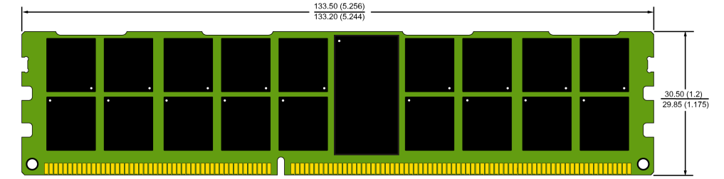
LR-DIMM MO-269 240 PIN
