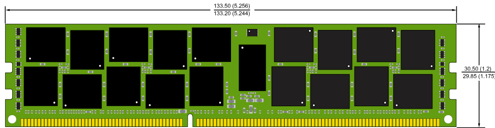
R-DIMM MO-269 240 PIN
