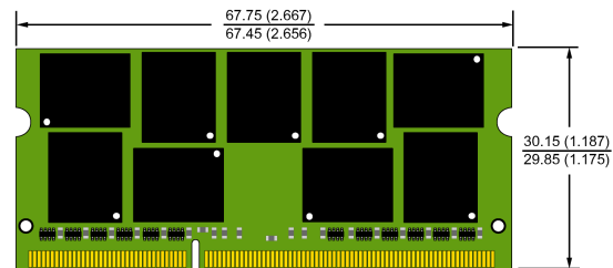
ECC SO-UDIMM JEDEC MO-268 204 PIN
